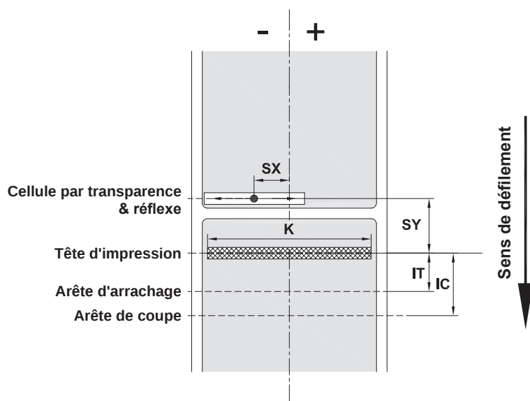
Figure 19 Dimensions
